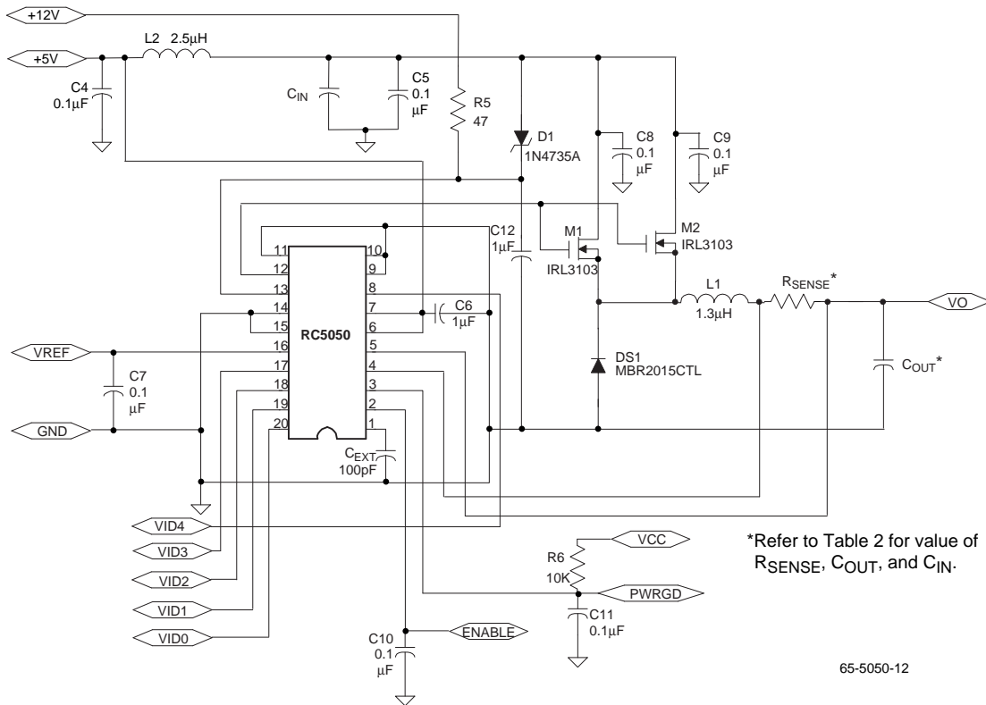
Figure 1. 15A Application Circuit for Pentium II Processor
